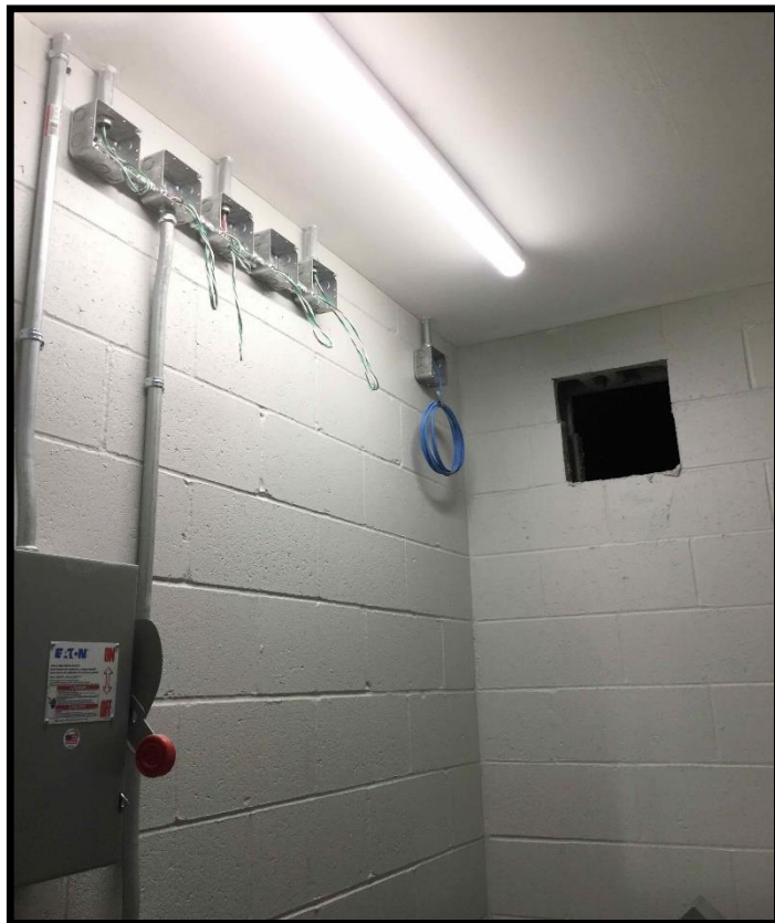
Elevator Machine Room
