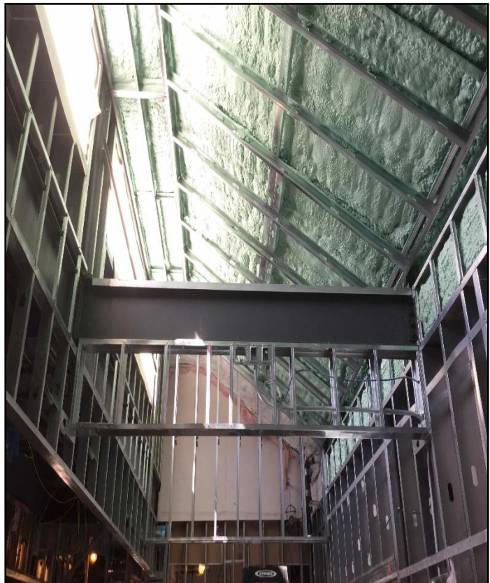
Meeting Room Insulation
