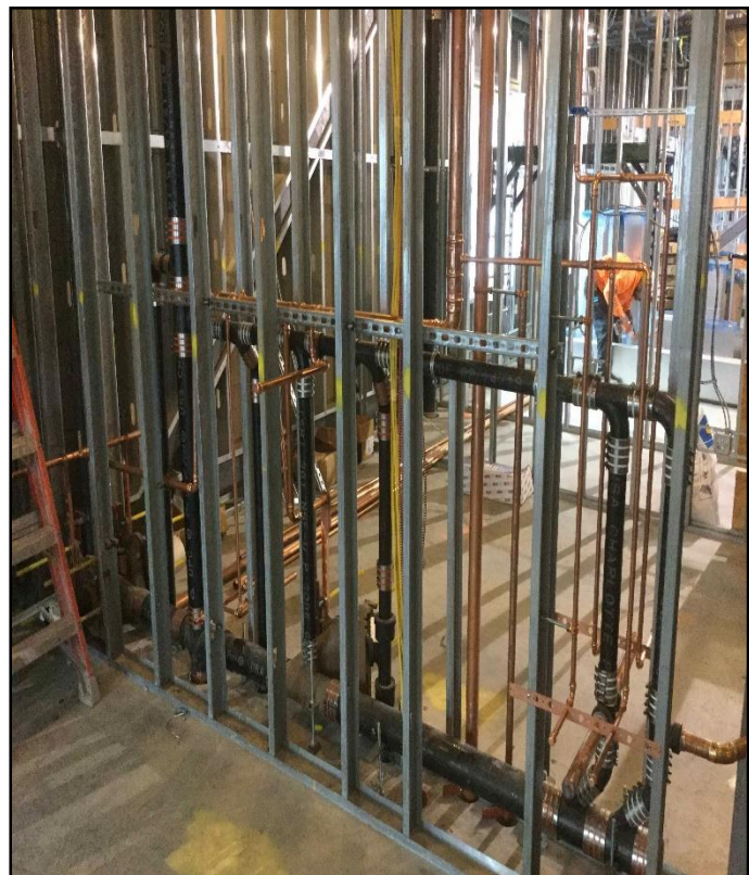
Bathroom Plumbing Rough
