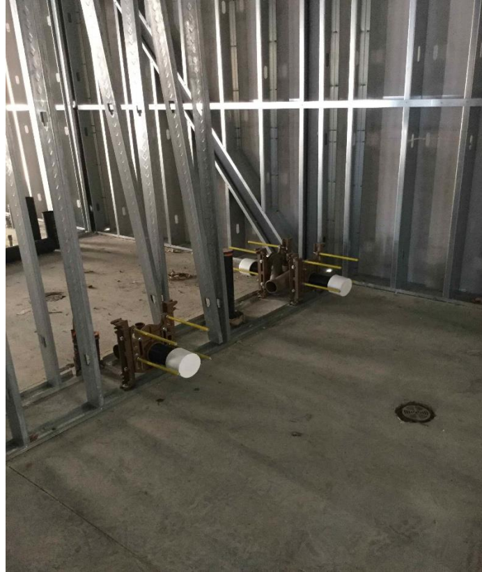
Rough Plumbing
