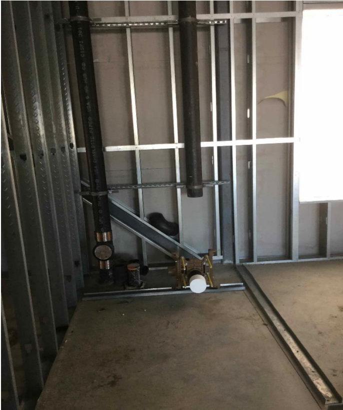
Rough Plumbing
