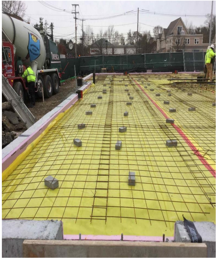
Slab Reinforcement
