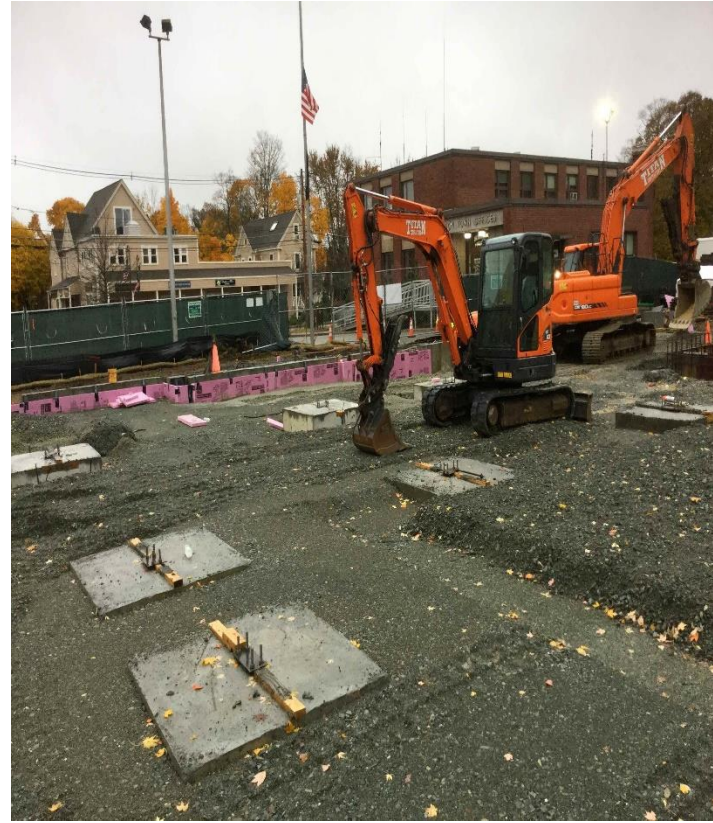
Interior Piers and Haunch
