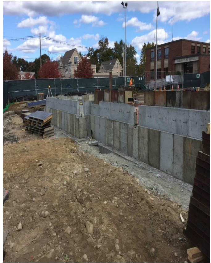
Strip Foundation Wall
